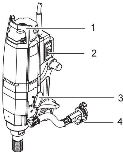
Operating elements
